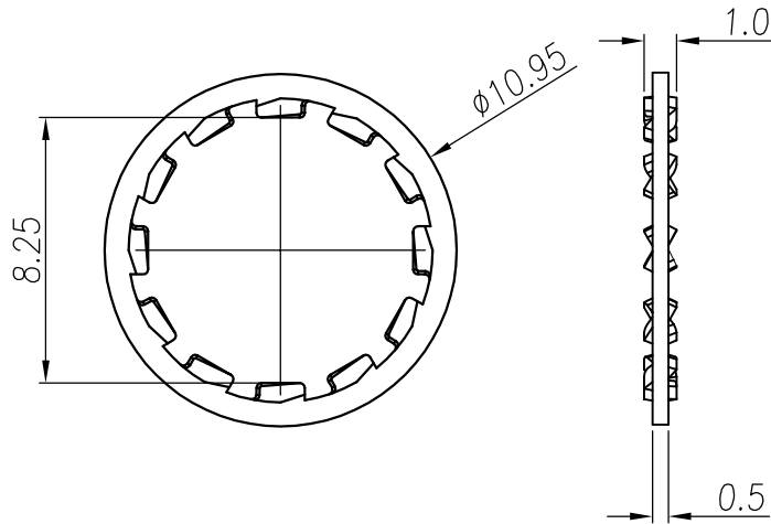
WASHER
