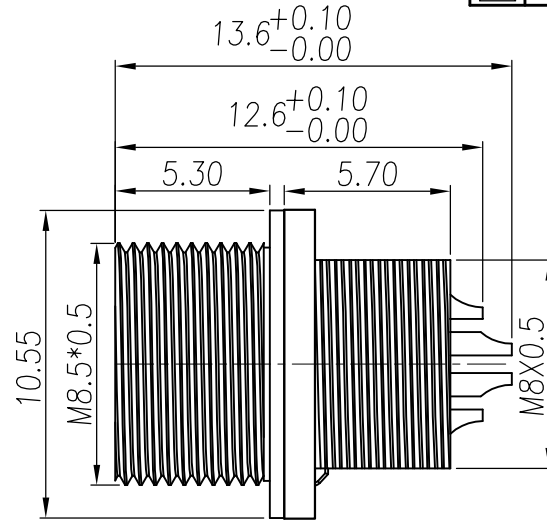
HOUSING+CONTACT+SHELL+O-RING
