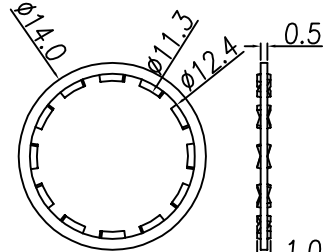
WASHER
