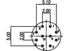
CONTACT ARRANGEMENT & DIMENSIONS(FRONT VIEW)
