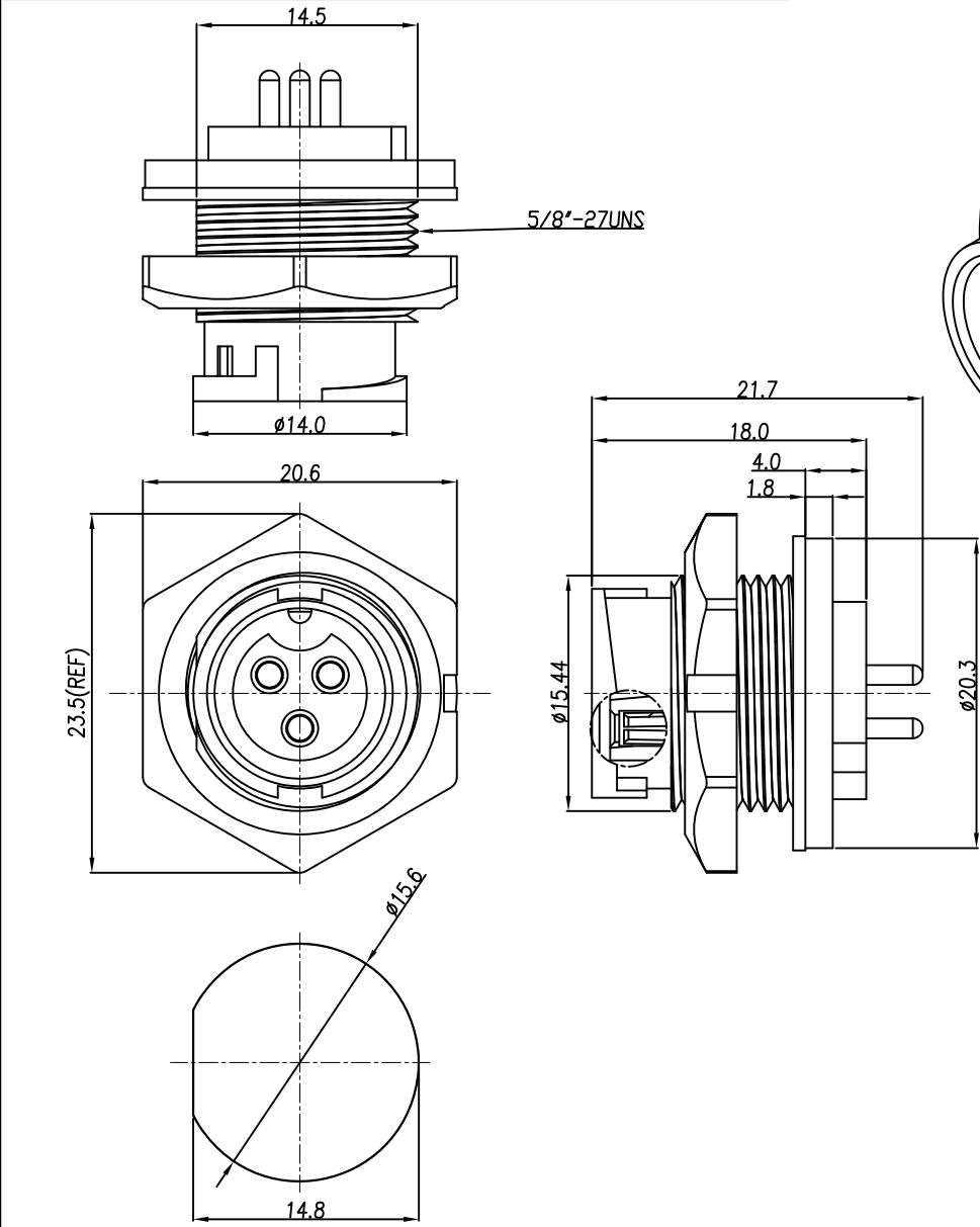
RECOMMENDED PANEL CUT-OUT
