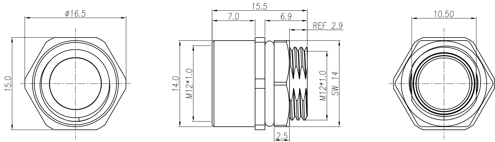
SHELL+O-RING A+NUT
