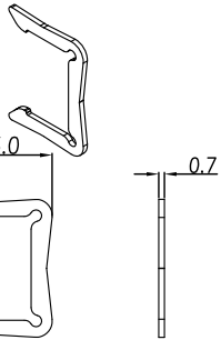
JAM MOUNT CLIP
