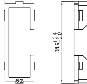
MOUNTING BRACKET 5-2
