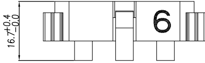
MOUNTING BRACKET 6
