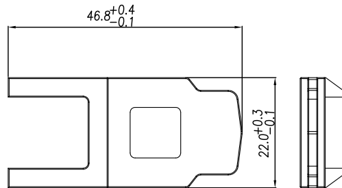
REMOVAL TOOL
