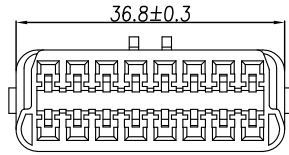
MAIN HOUSING
