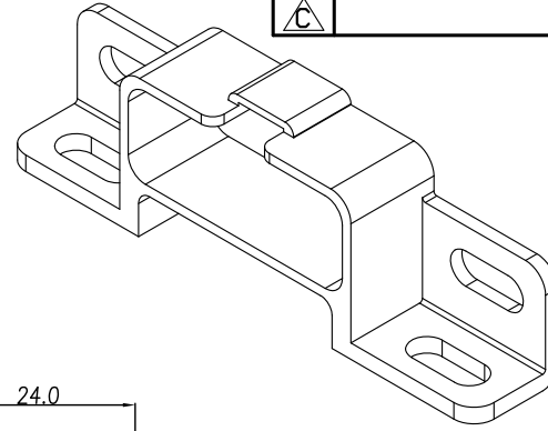
MOUNTING BRACKET 1
