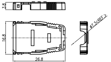
BOTTOM COVER HOUSING
