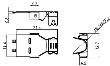
BACK SHELL OF PLUG
