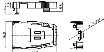
TOP COVER HOUSING
