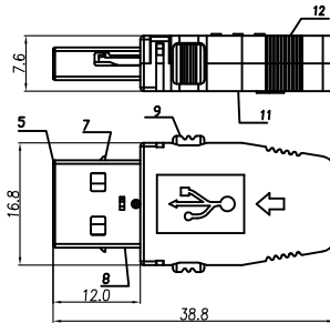
FRONT SHELL OF PLUG
