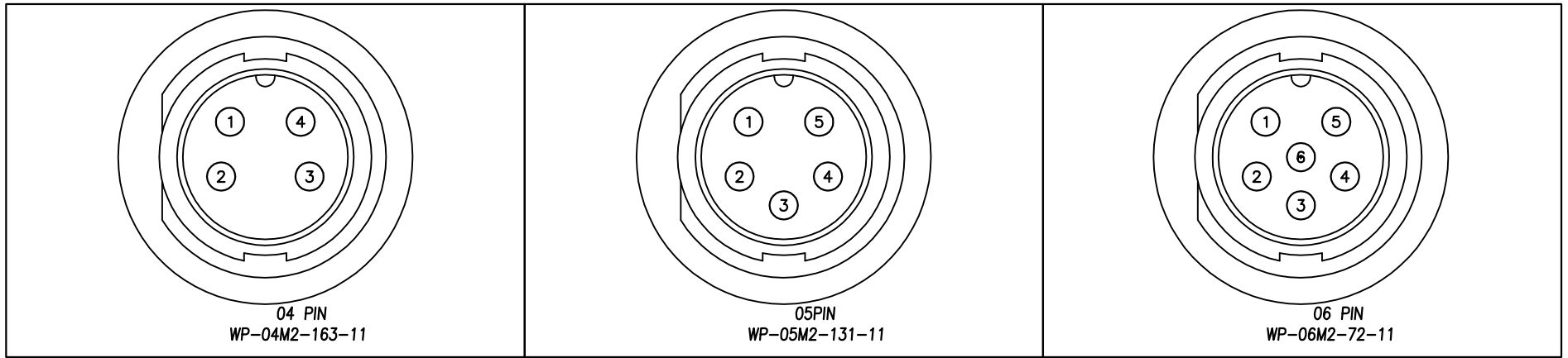
Pin Assignments Front View
